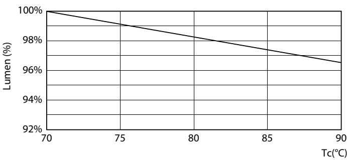
Lumen Maintenance Diagram - CorePro LED PLL EM/Mains 16.5W 830 4P
